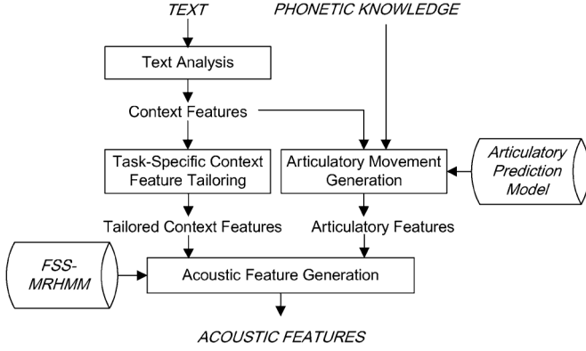
Fig. 4. Flowchart for the generation of acoustic features with articulatory control using the proposed Feature-Space-Switched MRHMM (FSS-MRHMM).
