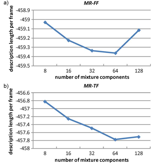
Fig. 7. Description length per frame on the training set with varying numbers of regression matrices for the a) MR-FF and b) MR-TF systems in the vowel identity modification task.
