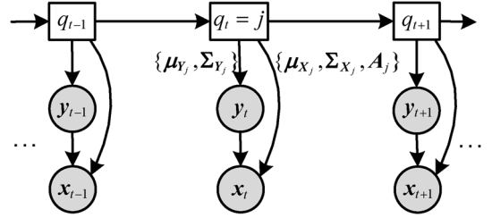
Fig. 1. Feature production model used in our previous unified acoustic-articulatory modelling method [12]. \mathbf{x}_t and \mathbf{y}_t are the acoustic and articulatory feature vectors respectively at frame t . The definition of the parameters on the arcs that represent the dependency relationship can be found in (3) and (4).
