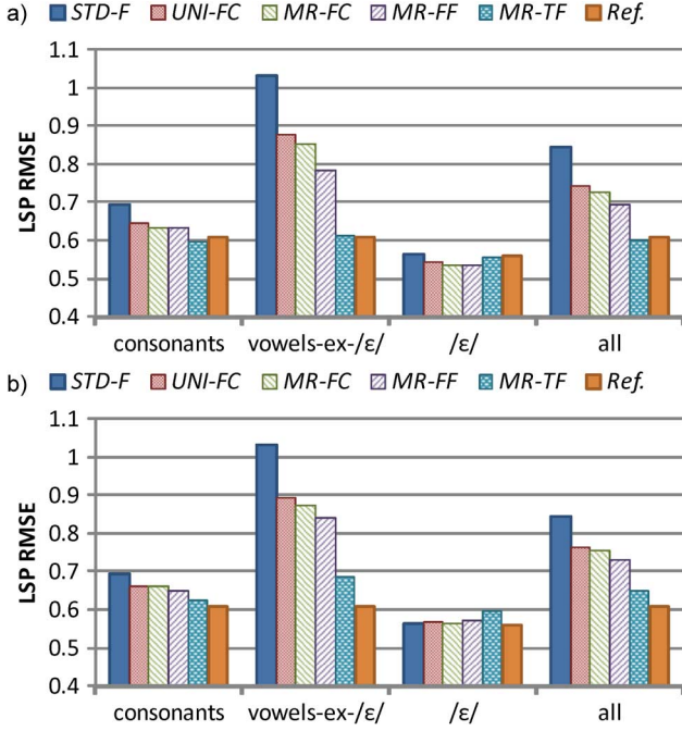
Fig. 8. LSP RMSEs for different systems and types of phone in the vowel identity modification experiment. “vowels-ex-/ε/” indicates all vowels excluding the source vowel /ε/ in the modification. The label Ref. represents the acoustic features generated using the STD-F system and the original context features without vowel replacement. For the UNI-FC , MR-FC , MR-FF , and MR-TF systems, the a) natural and b) generated articulatory features were used respectively.
