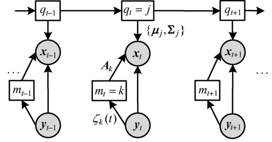
Fig. 6. Feature production model used in the MRHMM with feature-space regression matrix switching proposed here. \mathbf{x}_t and \mathbf{y}_t are the acoustic and articulatory feature vectors at frame t . The definition of the parameters on the arcs that represent the dependency relationship can be found in (10) and (11).
