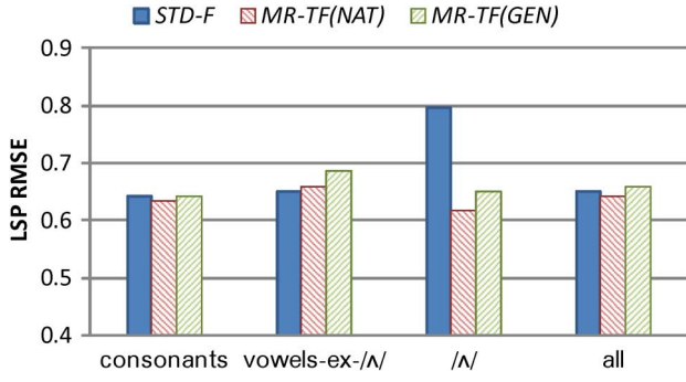
Fig. 11. LSP RMSEs for the STD - F and MR - TF systems in vowel creation experiment. “vowels-ex-/ʌ/” indicates all vowels excluding the source vowel /ʌ/. “NAT” and “GEN” in brackets denote the use of natural or generated articulatory features respectively.
