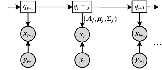
Fig. 5. Feature production model of the conventional MRHMM. \mathbf{x}_t and \mathbf{y}_t are the observed feature vector and auxiliary feature vector at frame t respectively. The definition of the parameters on the arcs that represent the dependency relationship can be found in (5) and (6).
