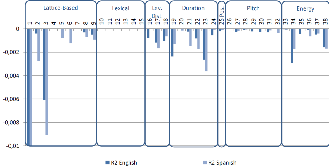
Figure 20: R^2 reduction with LR in the leave-one-out experiment for English and Spanish data on the verification set. “Lev. Dist.” refers to the Levenshtein distance-based features. “Pos.” stands for the Position feature.
